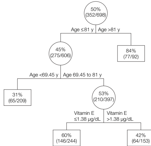
Figure 2. Classification Tree for Decline in Physical Performance Score
